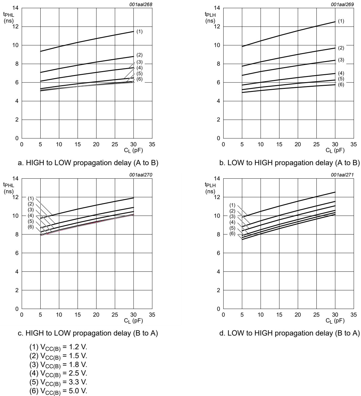
Fig. 6. Typical propagation delay versus load capacitance; T_{amb} = 25^\circ\text{C} ; V_{CC(A)} = 1.2 V
