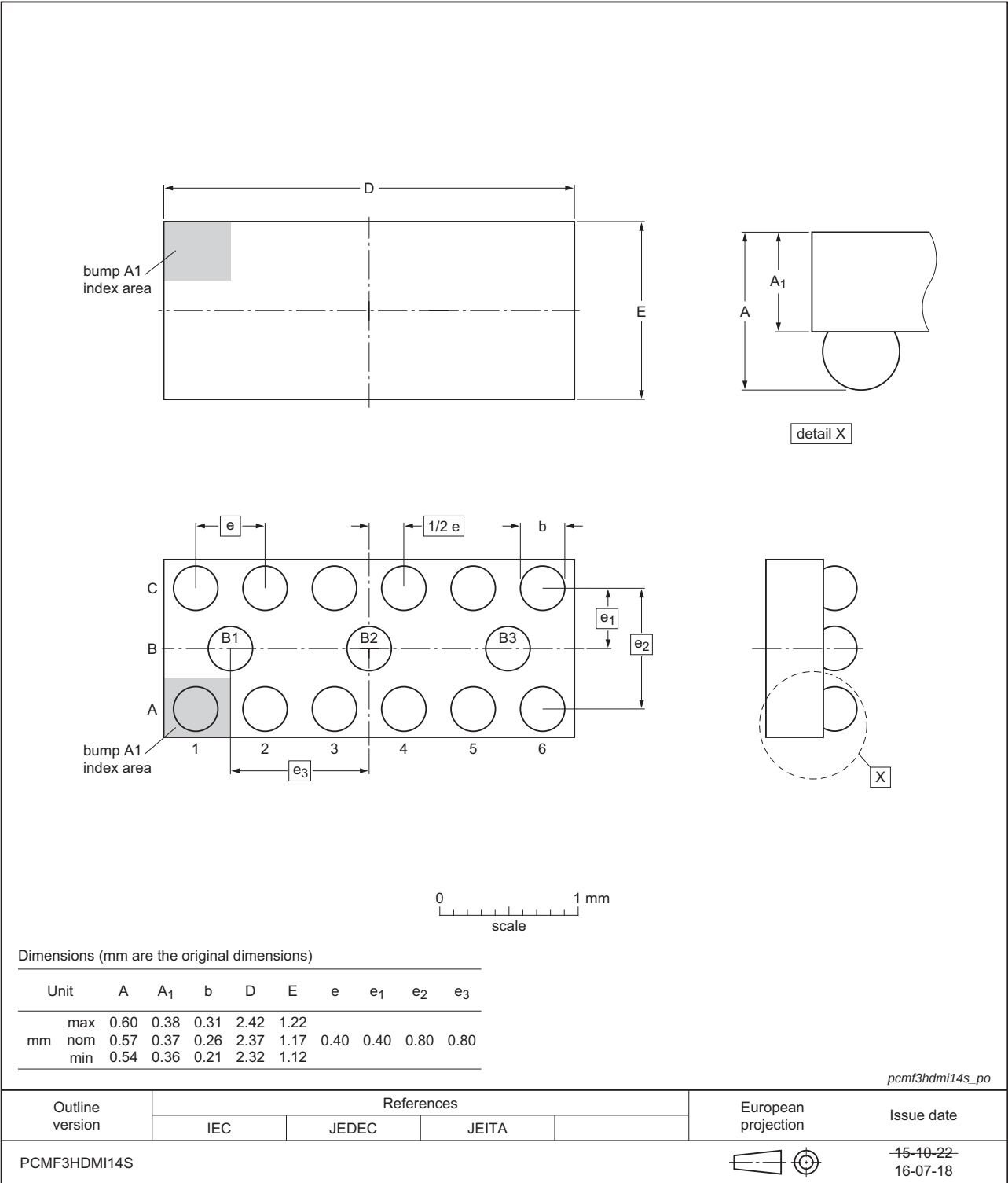
Fig 15. Package outline WLCSP15 (PCMF3HDMI14S)
