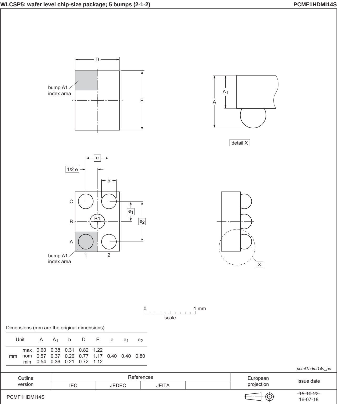
Fig 13. Package outline WLCSP5 (PCMF1HDMI14S)
