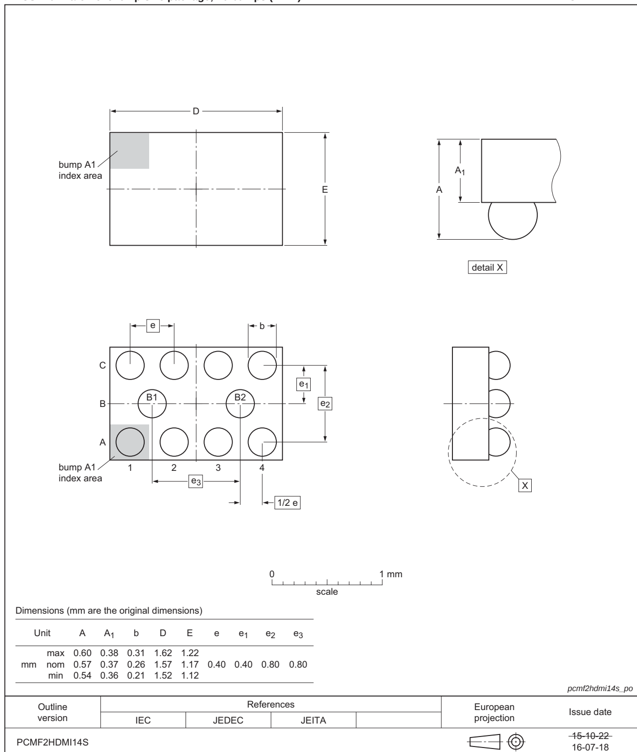
Fig 14. Package outline WLCSP10 (PCMF2HDMI14S)
