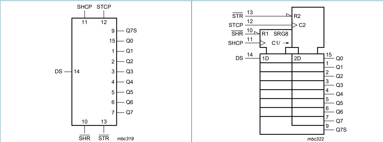
Fig. 2. Logic symbol
