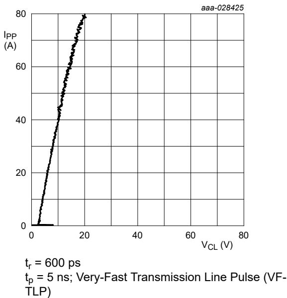
Fig. 13. Dynamic resistance with positive clamping; typical values
