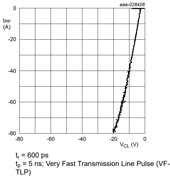
Fig. 14. Dynamic resistance with negative clamping; typical values
