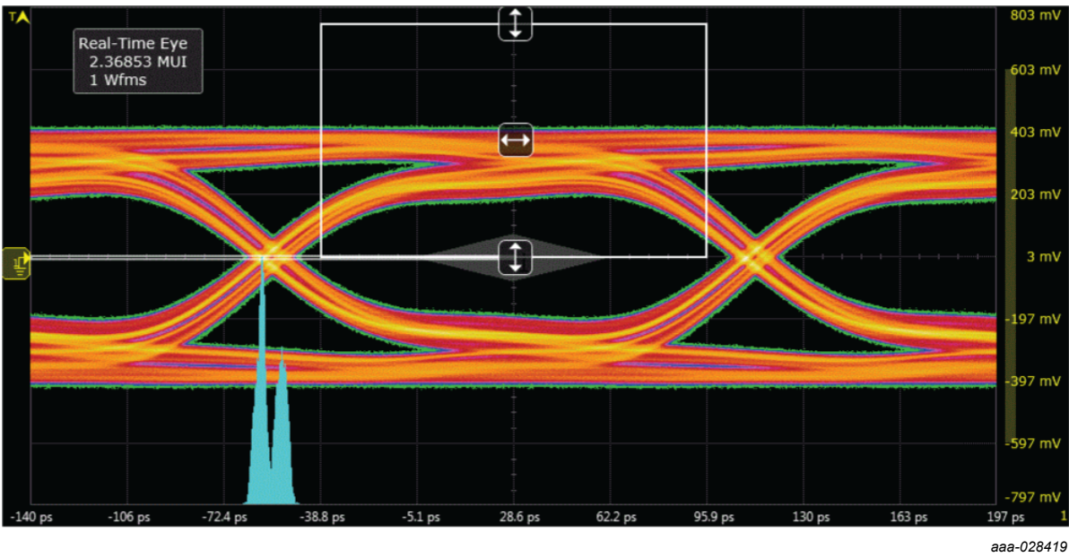
Fig. 7. HDMI TP1 eye diagram, PCB with device; typical values
