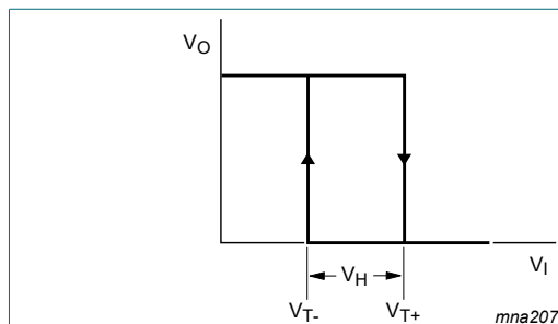
Fig. 6. Transfer characteristic
