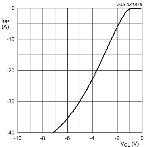
Fig. 6. Dynamic resistance with negative clamping; typical values
