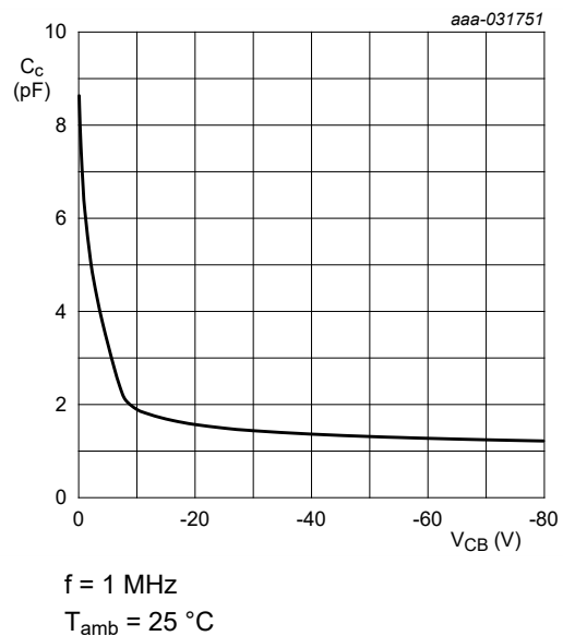
Fig. 14. NHUMB13: Collector capacitance as a function of collector-base voltage; typical values
