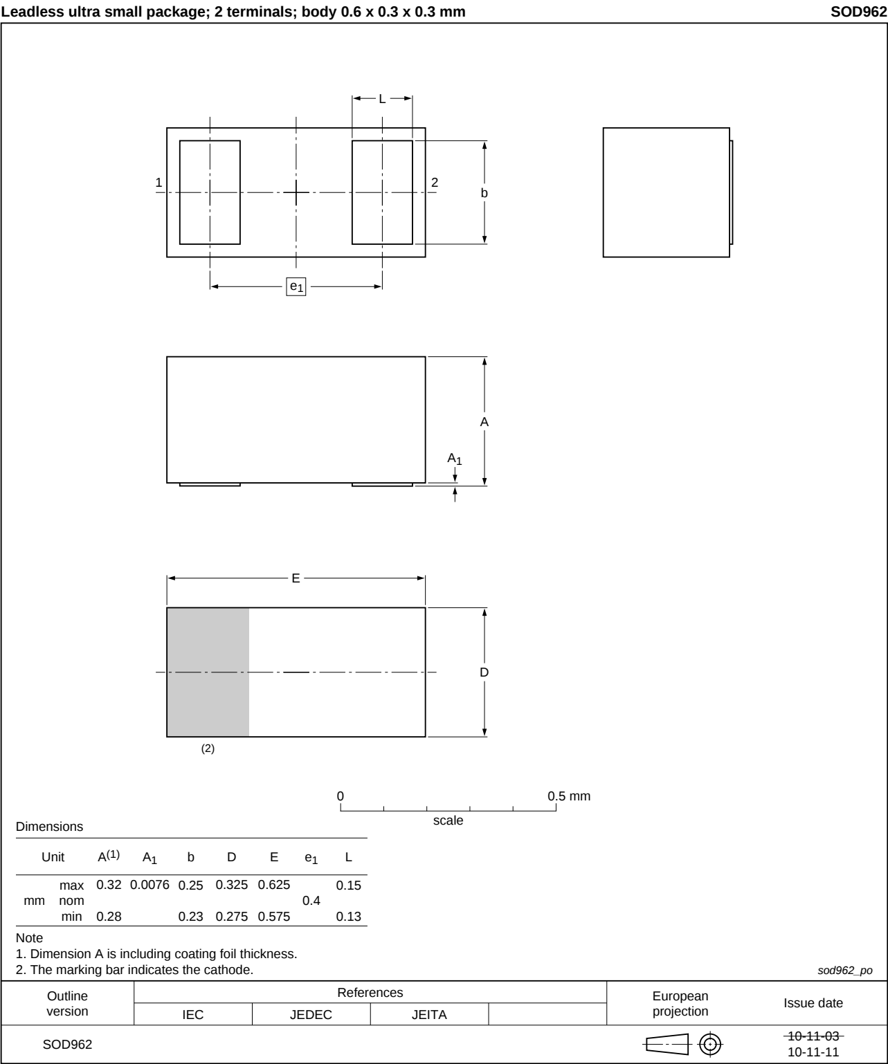
Fig 9. Package outline PESD5V0V1BCSF (SOD962)
