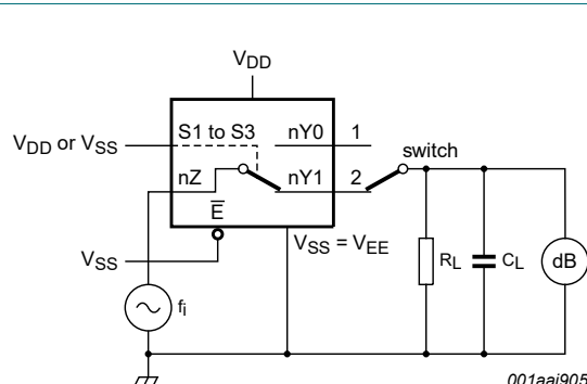
Fig. 17. Test circuit for measuring frequency response
