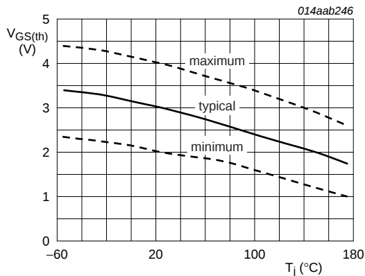
Fig 10. Gate-source threshold voltage as a function of junction temperature
