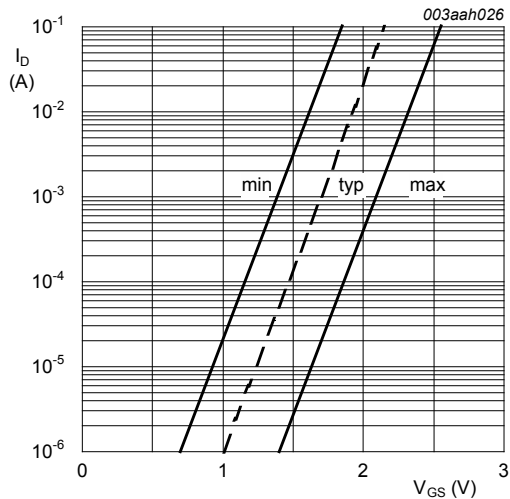
Fig. 11. Sub-threshold drain current as a function of gate-source voltage T_J = 25\text{ }^{\circ}\text{C}; V_{DS} = 5\text{ V}
