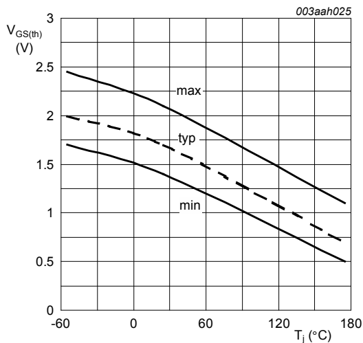
Fig. 10. Gate-source threshold voltage as a function of junction temperature I_D = 1\text{ mA}; V_{DS} = V_{GS}
