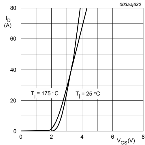
Fig. 9. Transfer characteristics; drain current as a function of gate-source voltage; typical values V_{DS} = 10\text{ V}
