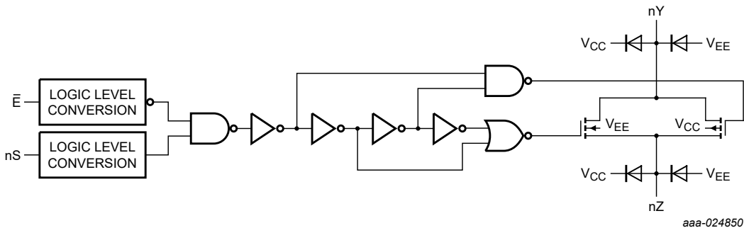
Fig. 4. Schematic diagram (one switch)
