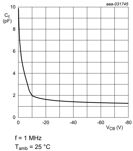
Fig. 14. NHUMD10, TR2 (PNP): Collector capacitance as a function of collector-base voltage; typical values
