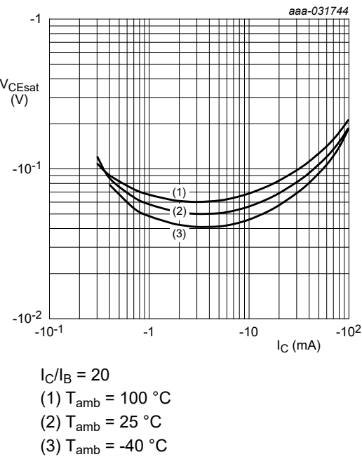
Fig. 13. NHUMD10, TR2 (PNP): Collector-emitter saturation voltage as a function of collector current; typical values
