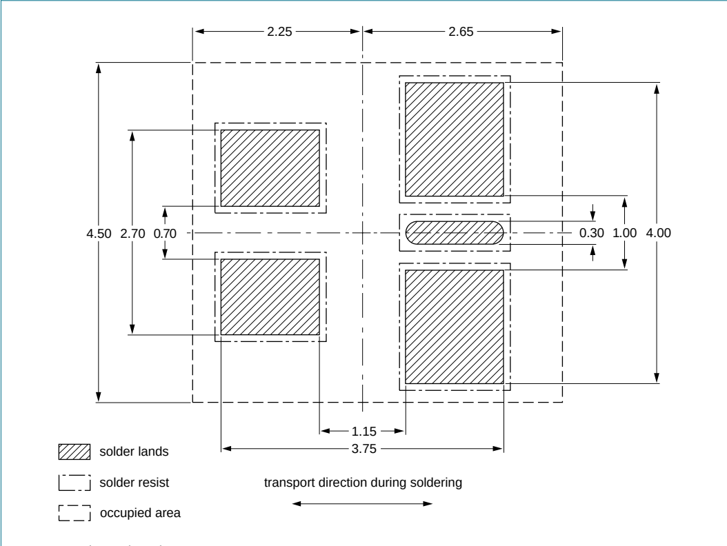
Fig 9. Wave soldering footprint SOT353 (SC-88A)
