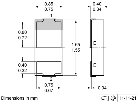
Fig. 17. Package outline DFN1608D-2 (SOD1608)
