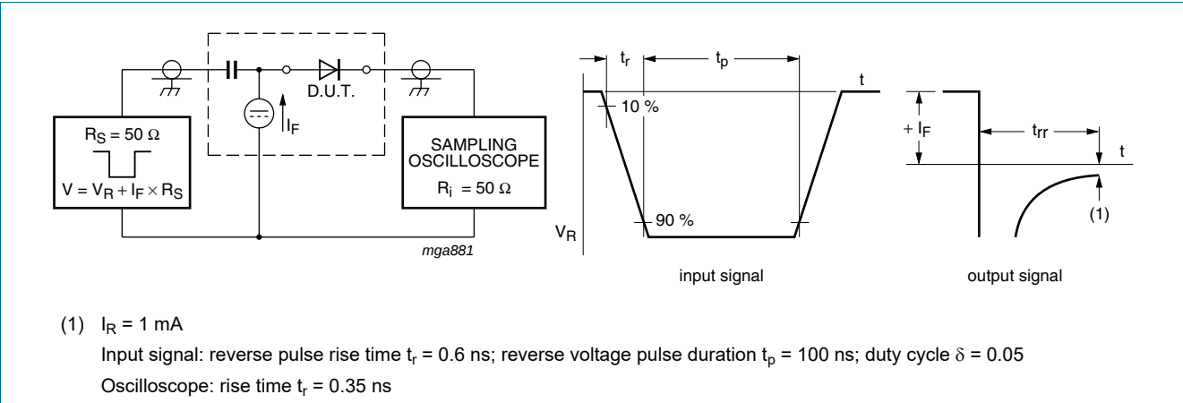
Fig 6. Reverse recovery time test circuit and waveforms
