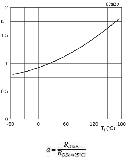
Fig 9. Normalized drain-source on-state resistance factor as a function of junction temperature
