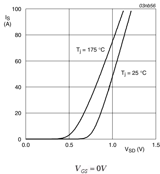
Fig 15. Reverse diode current; typical value
