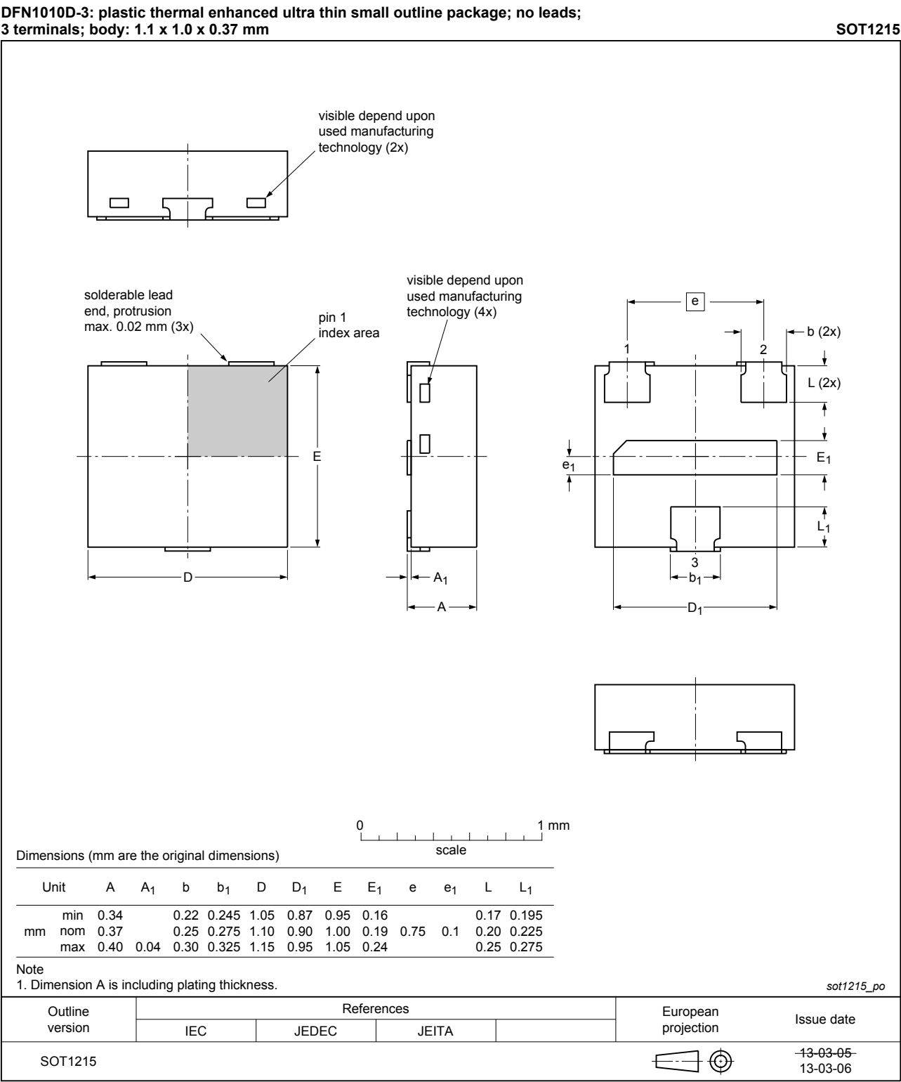
Fig. 11. Package outline DFN1010D-3 (SOT1215)
