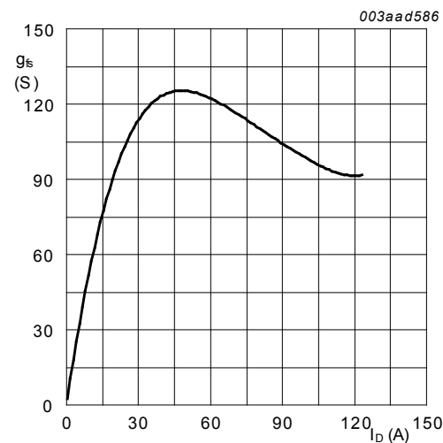
Fig. 8. Forward transconductance as a function of drain current; typical values T_j = 25\text{ }^{\circ}\text{C}; V_{DS} = 15\text{ V}
