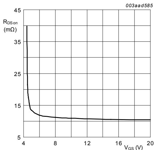
Fig. 7. Drain-source on-state resistance as a function of gate-source voltage; typical values T_j = 25\text{ }^{\circ}\text{C}
