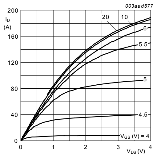
Fig. 5. Output characteristics: drain current as a function of drain-source voltage; typical values T_j = 25\text{ }^{\circ}\text{C}
