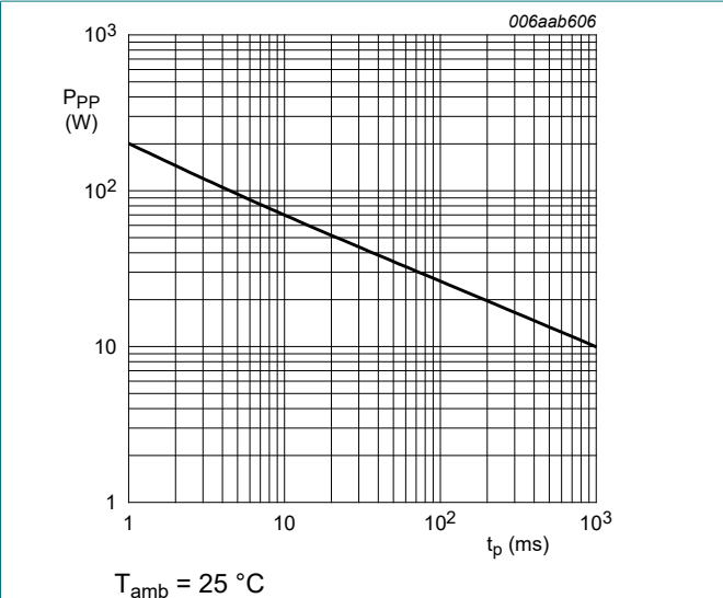
Fig. 3. Peak pulse power as a function of exponential pulse duration; typical values
