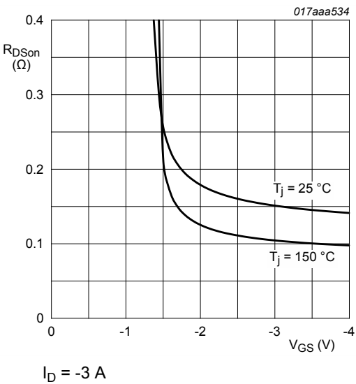
Fig. 11. MOSFET transistor: Drain-source on-state resistance as a function of gate-source voltage; typical values
