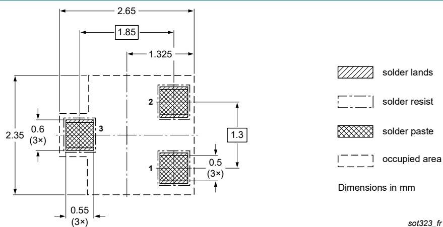
Fig. 15. Reflow soldering footprint SOT323 (SC-70)
