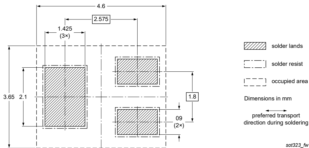
Fig. 16. Wave soldering footprint SOT323 (SC-70)
