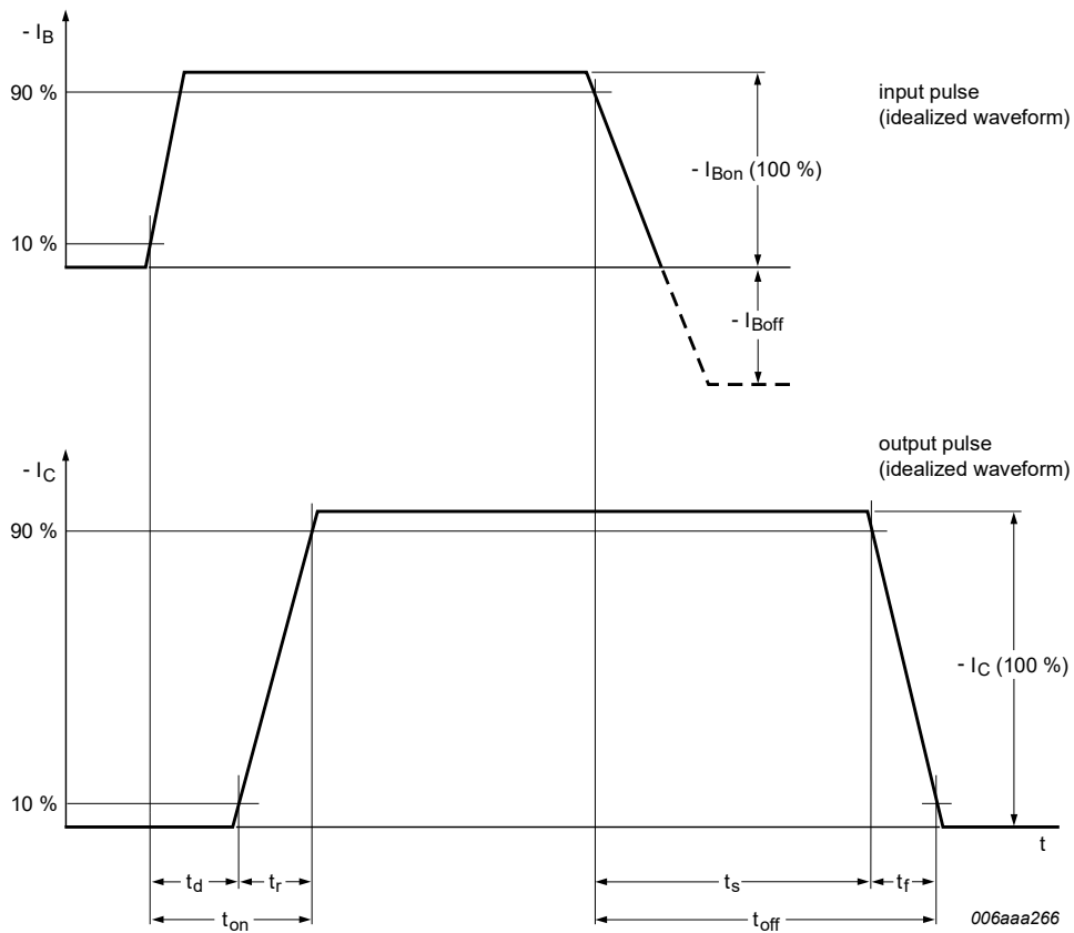
Fig. 8. BISS transistor switching time definition
