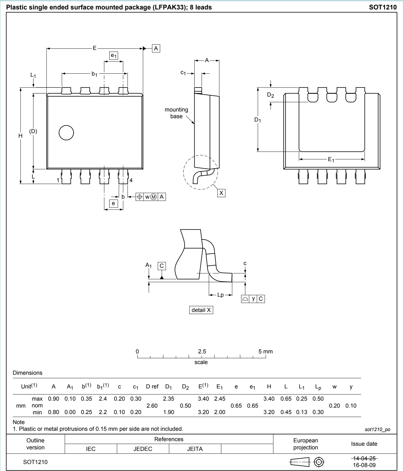
Fig. 17. Package outline LFPAK33 (SOT1210)
