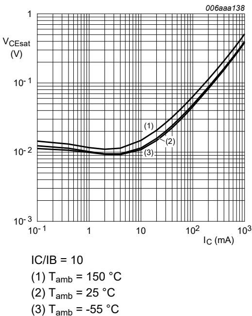
Fig. 11. BC817-25QC-Q: Collector-emitter saturation voltage as a function of collector current; typical values
