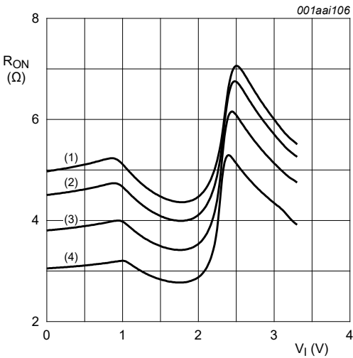
Fig. 10. ON resistance as a function of input voltage; V_{CC} = 3.3 V; I_{SW} = 24 mA
