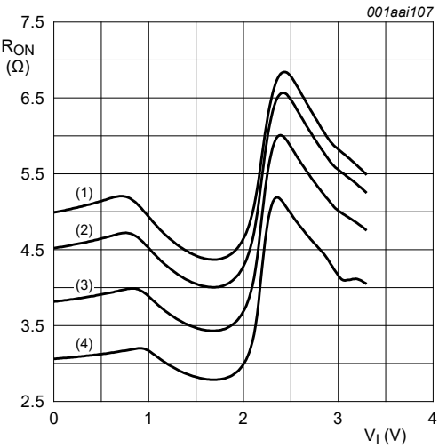
Fig. 11. ON resistance as a function of input voltage; V_{CC} = 3.3 V; I_{SW} = 64 mA
