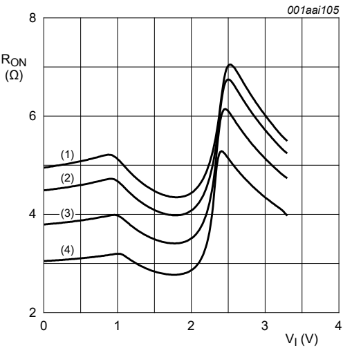
Fig. 9. ON resistance as a function of input voltage; V_{CC} = 3.3 V; I_{SW} = 15 mA
