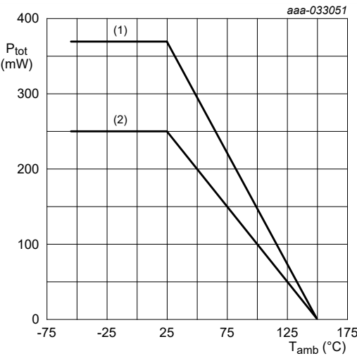
(1) FR4 PCB, single-sided, 35 μm copper, tin-plated, mounting pad for collector 1 cm 2 (2) FR4 PCB, single-sided, 35 μm copper, tin-plated and standard footprint
