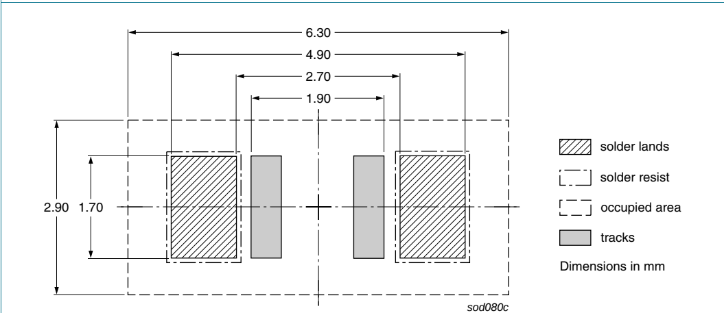
Fig 7. Wave soldering footprint SOD80C
