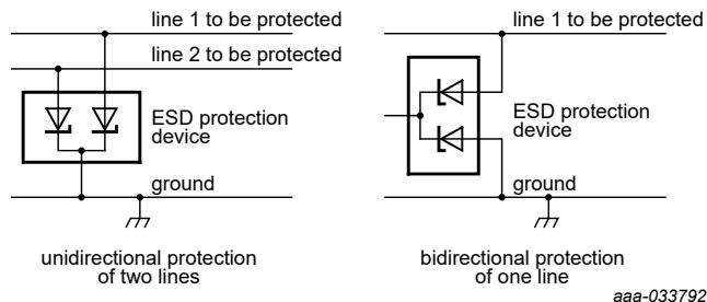
Fig. 8. Typical application: ESD protection of data lines
