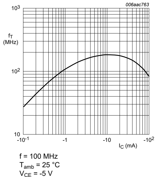
Fig. 16. PNP transistor: Transition frequency as a function of collector current; typical values of built-in transistor
