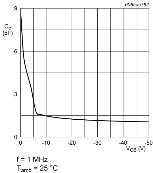
Fig. 15. PNP transistor: Collector capacitance as a function of collector-base voltage; typical values
