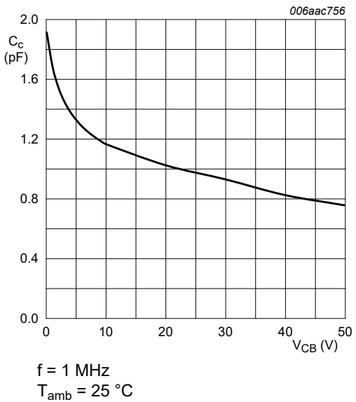
Fig. 8. NPN transistor: Collector capacitance as a function of collector-base voltage; typical values
