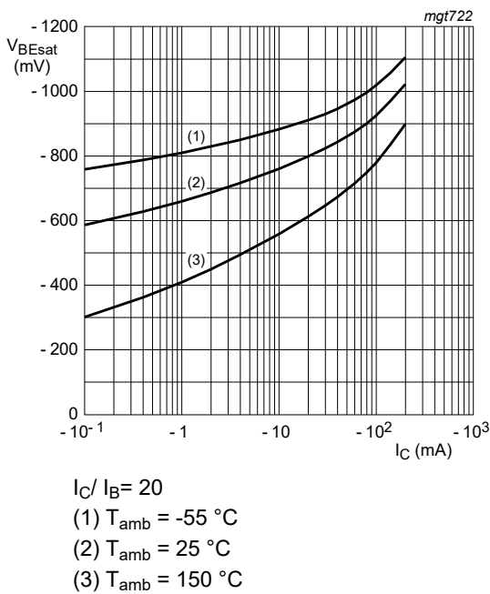
Fig. 15. BC857CQB: Base-emitter saturation voltage as a function of collector current; typical values
