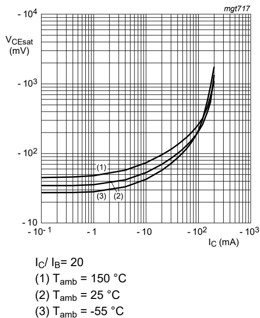
Fig. 10. BC857BQB: Collector-emitter saturation voltage as a function of collector current; typical values
