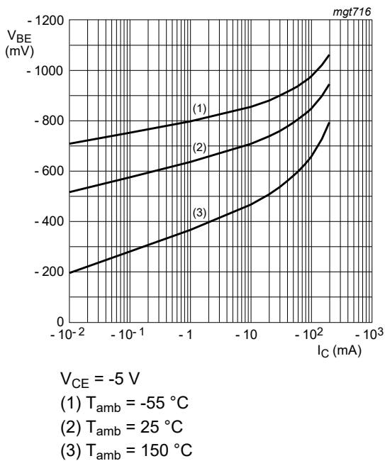
Fig. 9. BC857BQB: Base-emitter voltage as a function of collector current; typical values
