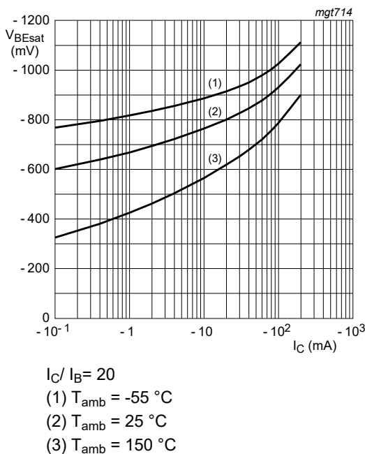
Fig. 7. BC857AQB: Base-emitter saturation voltage as a function of collector current; typical values
