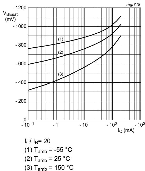
Fig. 11. BC857BQB: Base-emitter saturation voltage as a function of collector current; typical values
