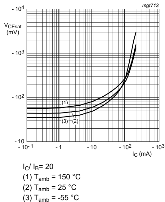
Fig. 6. BC857AQB: Collector-emitter saturation voltage as a function of collector current; typical values
