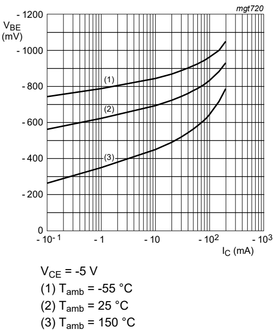
Fig. 13. BC857CQB: Base-emitter voltage as a function of collector current; typical values
