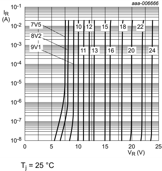
Fig. 9. Reverse current as a function of reverse voltage; typical values (BZX384-A/B/C7V5-Q to BZX384-A/B/C24-Q)
