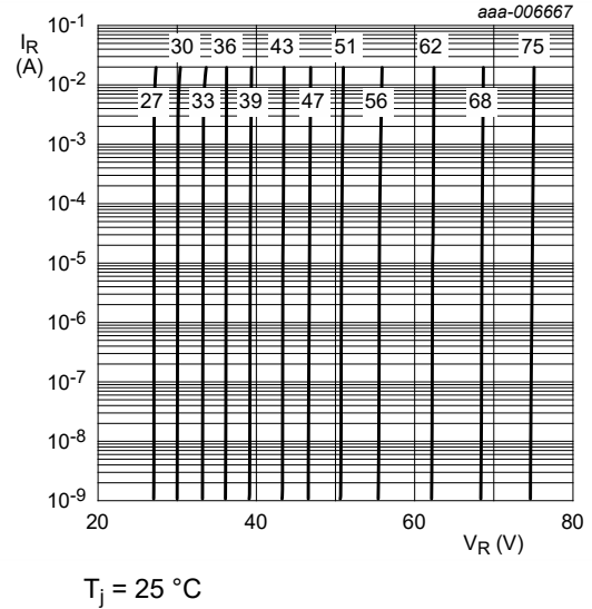
Fig. 10. Reverse current as a function of reverse voltage; typical values (BZX384-A/B/C27-Q to BZX384-A/B/C75-Q)
