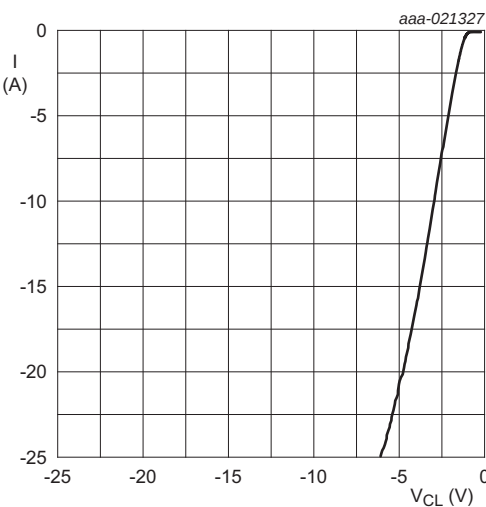
Fig 9. Dynamic resistance with negative clamping; typical values
