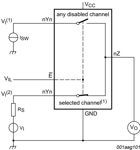
Fig. 5. Test circuit for measuring ON-state leakage current
