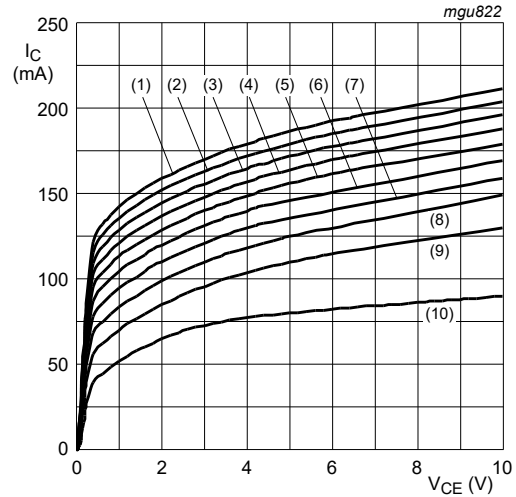
T_{amb} = 25\text{ }^{\circ}\text{C} (1) I_B = 5.0\text{ mA} (2) I_B = 4.5\text{ mA} (3) I_B = 4.0\text{ mA} (4) I_B = 3.5\text{ mA} (5) I_B = 3.0\text{ mA} (6) I_B = 2.5\text{ mA} (7) I_B = 2.0\text{ mA} (8) I_B = 1.5\text{ mA} (9) I_B = 1.0\text{ mA} (10) I_B = 0.5\text{ mA}
