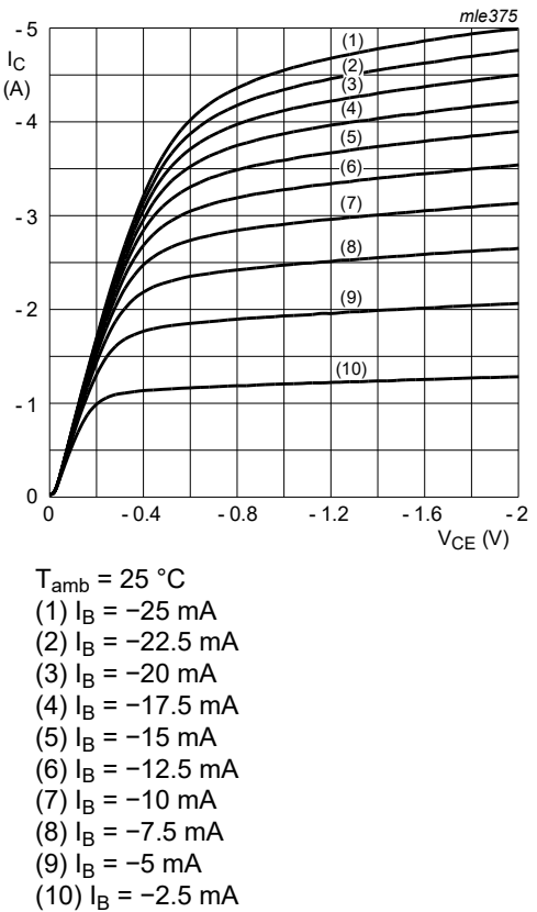
Fig. 11. Collector current as a function of collector-emitter voltage; typical values
