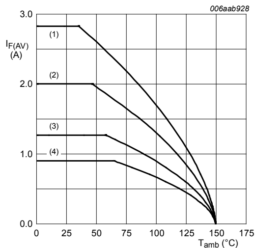
FR4 PCB, mounting pad for cathode 1\text{ cm}^2 T_j = 150\text{ }^{\circ}\text{C} (1) \delta = 1 ; DC (2) \delta = 0.5 ; f = 20\text{ kHz} (3) \delta = 0.2 ; f = 20\text{ kHz} (4) \delta = 0.1 ; f = 20\text{ kHz}
