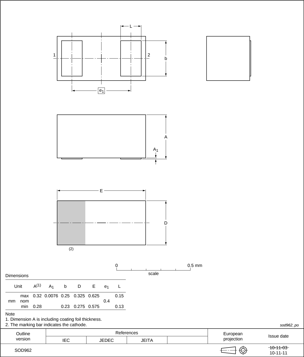
Fig 11. Package outline PESD5V0S1BSF (SOD962)
