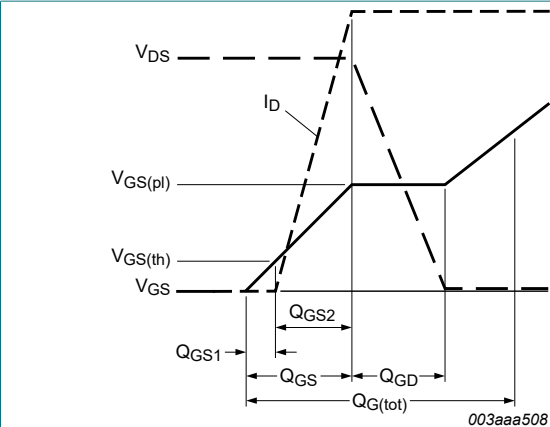
Fig. 13. Gate charge waveform definitions
