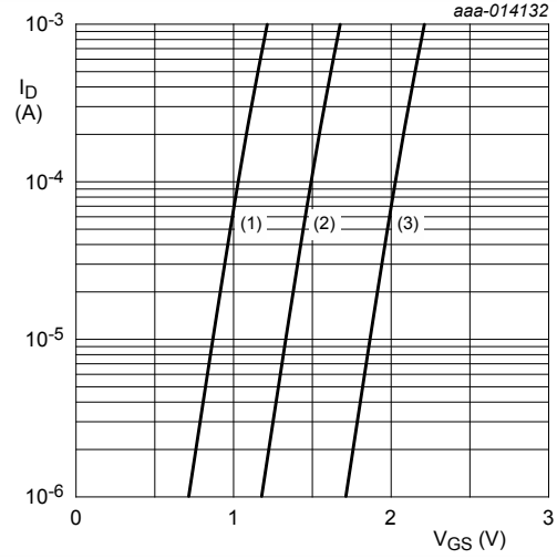
Fig. 8. Sub-threshold drain current as a function of gate-source voltage T_j = 25^\circ\text{C}; V_{DS} = 5 (1) minimum values (2) typical values (3) maximum values
