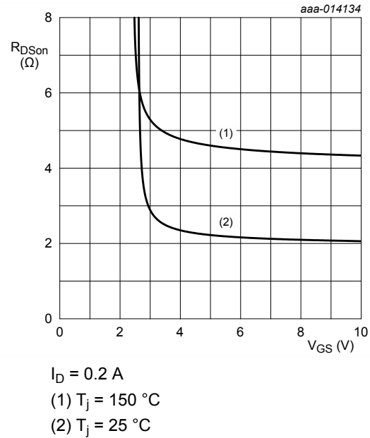
Fig. 10. Drain-source on-state resistance as a function of gate-source voltage; typical values I_D = 0.2 A (1) T_j = 150^\circ\text{C} (2) T_j = 25^\circ\text{C}
