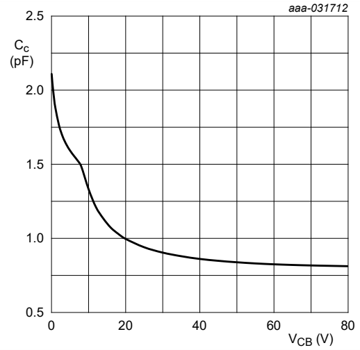
Fig. 32. NHUMD12, TR1 (NPN): Collector capacitance as a function of collector-base voltage; typical values
