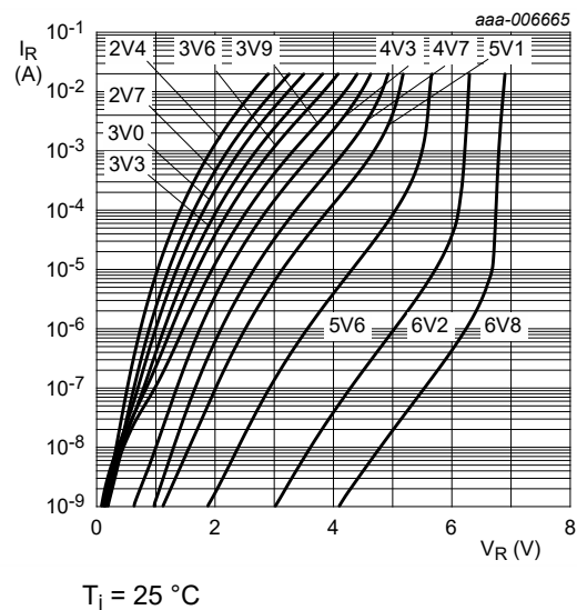
Fig. 8. Reverse current as a function of reverse voltage; typical values (BZX84J-B/C2V4-Q to B/C6V8-Q)
