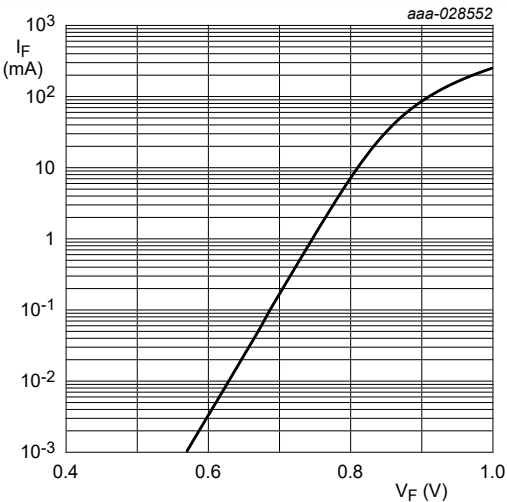
Fig. 4. Forward current as a function of forward voltage; typical values (BZX84J-B/C7V5-Q)
