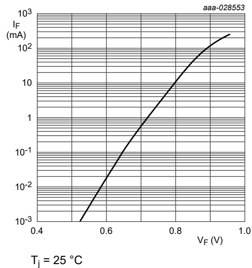
Fig. 5. Forward current as a function of forward voltage; typical values (BZX84J-B/C75-Q)
