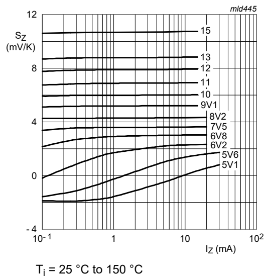
Fig. 7. Temperature coefficient as a function of working current; typical values (BZX84J-B/C5V1-Q to B/C15-Q)
