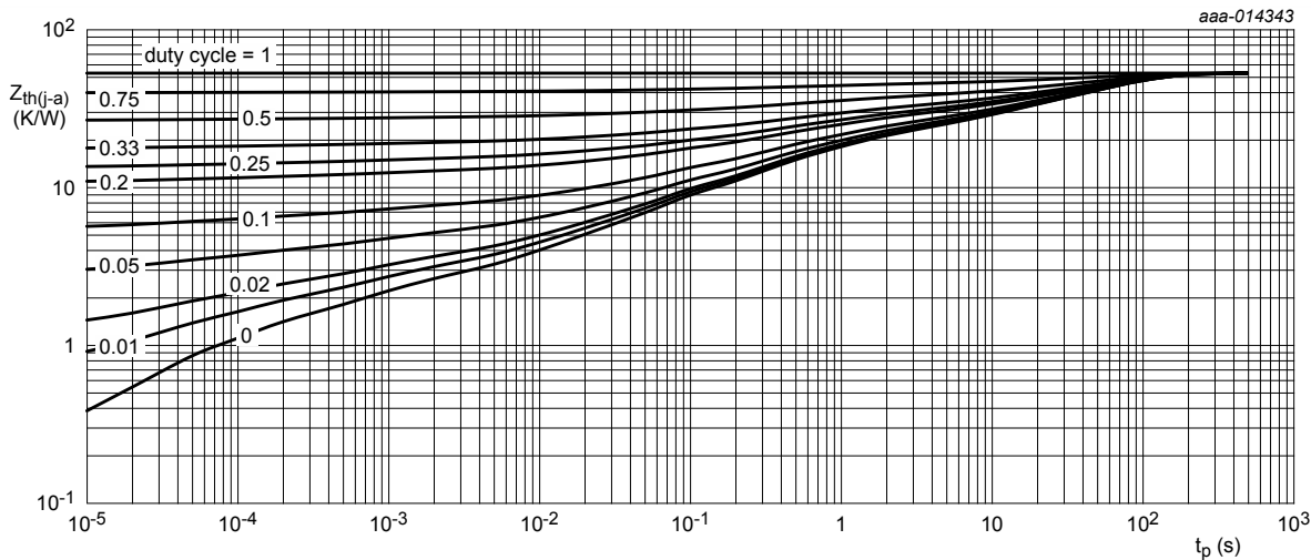
FR4 PCB, mounting pad for collector 6 cm 2 Fig. 3. Per transistor: transient thermal impedance from junction to ambient as a function of pulse duration; typical values
