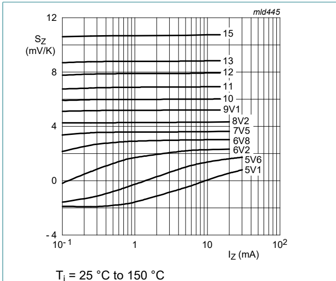
Fig. 7. Temperature coefficient as a function of working current; typical values (BZT52H-A/B/C5V1-Q to BZT52H-A/B/C15-Q)
