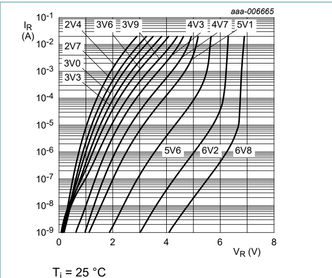
Fig. 8. Reverse current as a function of reverse voltage; typical values (BZT52H-A/B/C2V4-Q to BZT52H-A/B/C6V8-Q)
