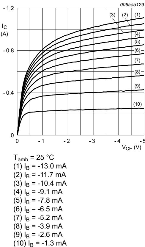
Fig. 7. Collector current as a function of collector-emitter voltage; typical values
