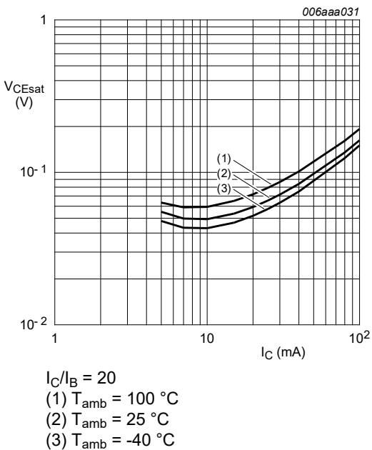
Fig. 10. TR2 (NPN): Collector-emitter saturation voltage as a function of collector current; typical values
