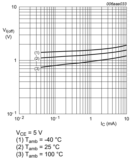
Fig. 12. TR2 (NPN): Off-state input voltage as a function of collector current; typical values
