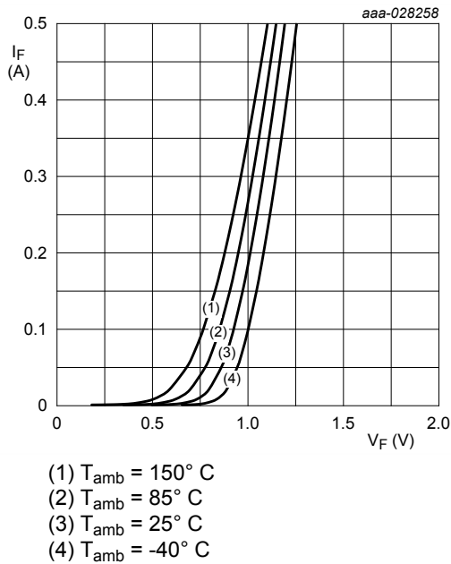
Fig. 3. Forward current as a function of forward voltage; typical values; (linear scale)
