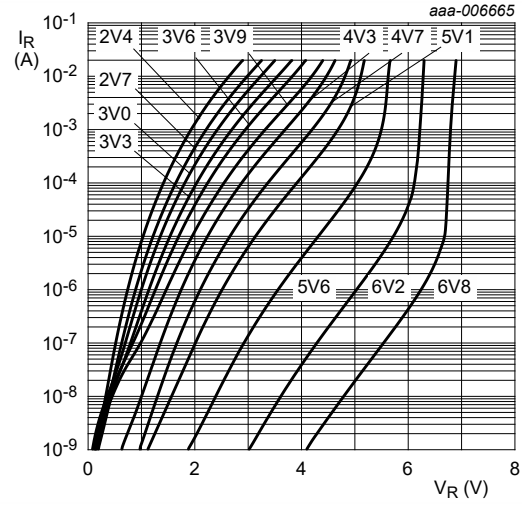
Fig. 8. Reverse current as a function of reverse voltage; typical values (BZT52H-A/B/C2V4 to BZT52H-A/B/C6V8)
