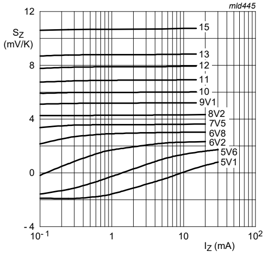
Fig. 7. Temperature coefficient as a function of working current; typical values (BZT52H-A/B/C5V1 to BZT52H-A/B/C15)
