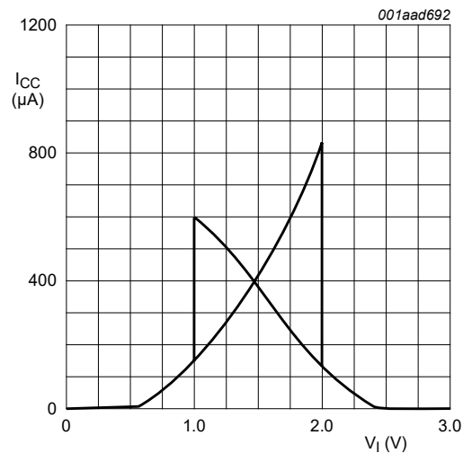
Fig. 9. Typical transfer characteristics; V_{CC} = 3.0\text{ V}
